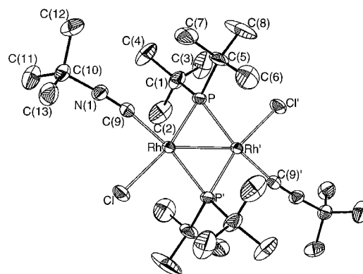
Figure 1. Molecular structure of 4b (hydrogen atoms omitted; primed atoms are related to the unprimed ones by an inversion center). Selected bond lengths [ \text{\AA} ] and angles [ ^\circ ]: \text{Rh-Rh}' 2.7583(6), \text{Rh-P} 2.2168(10), \text{Rh-P}' 2.2705(10), \text{Rh-Cl} 2.3962(10), \text{Rh-C(9)} 1.992(4); \text{P-Rh-P}' 104.15(3), \text{P-Rh-Cl} 167.22(4), \text{P-Rh-C(9)} 88.67(11), \text{P'-Rh-Cl} 88.00(4), \text{P'-Rh-C(9)} 166.92(11), \text{Cl-Rh-C(9)} 79.41(11), \text{Rh'-Rh-P} 52.96(3), \text{Rh'-Rh-P'} 51.20(3), \text{Rh'-Rh-Cl} 139.02(3), \text{Rh'-Rh-C(9)} 141.55(11), \text{Rh-P-Rh}' 75.85(3).
